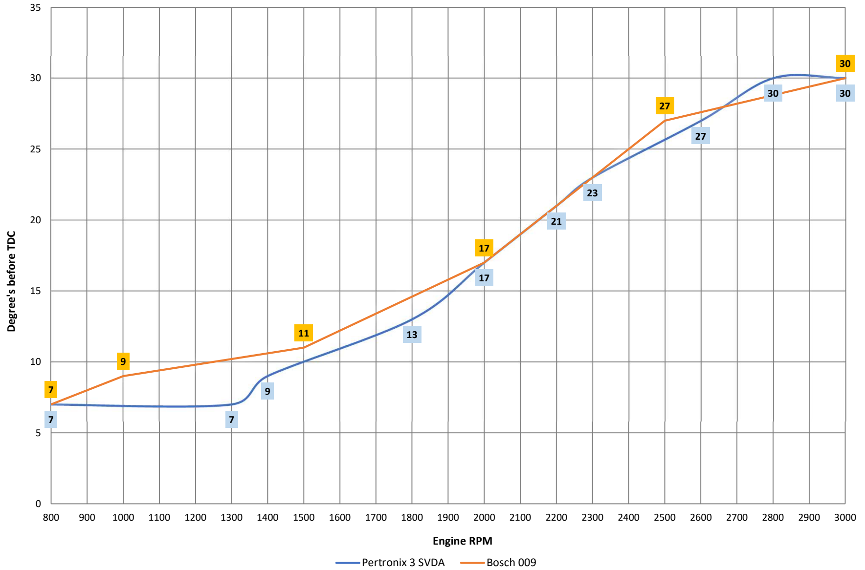
Distributor Mechanical Advance related to engine RPM
