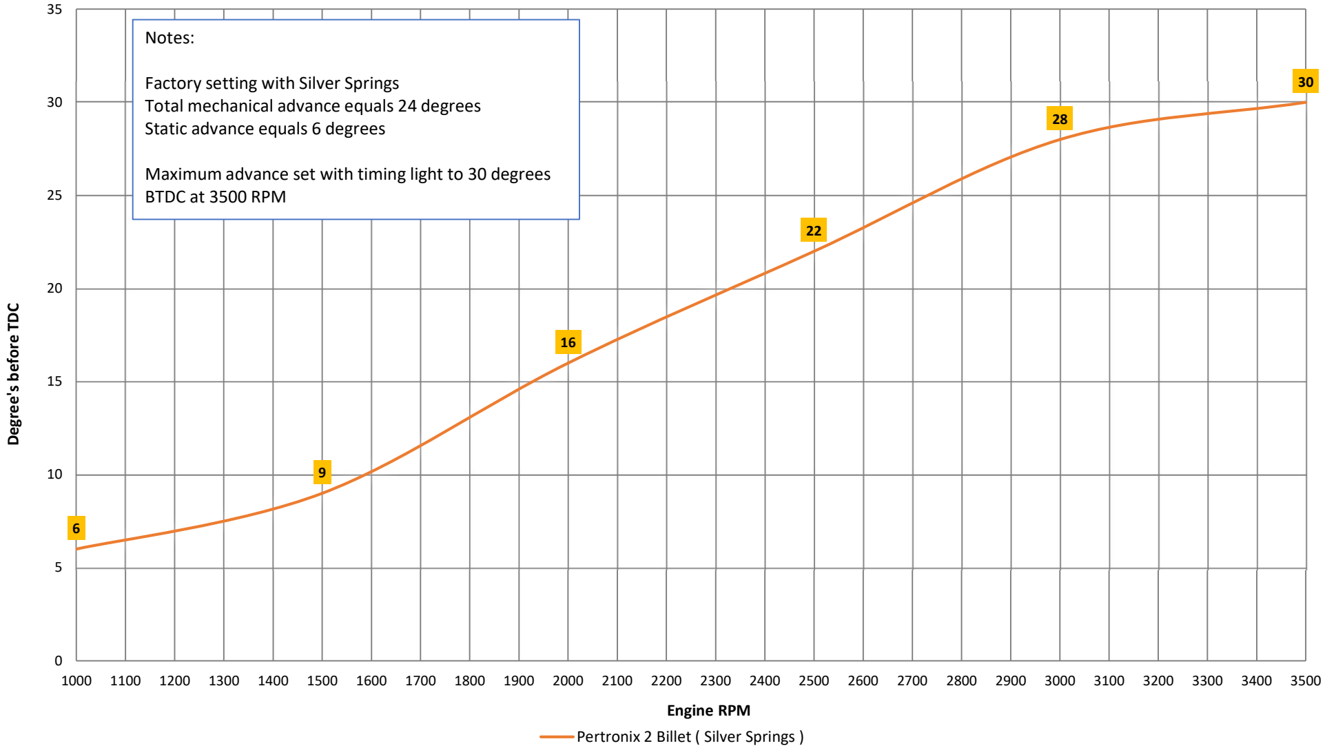
Distributor Mechanical Advance related to engine RPM
